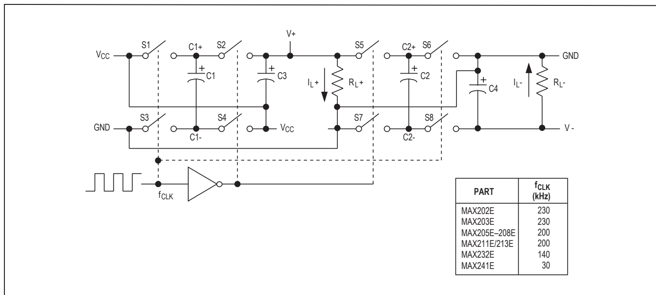
Figure 4. Charge-Pump Diagram
