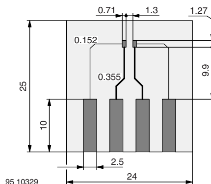
Fig. 5 - Board for R_{\theta JA} Definition (in mm)
